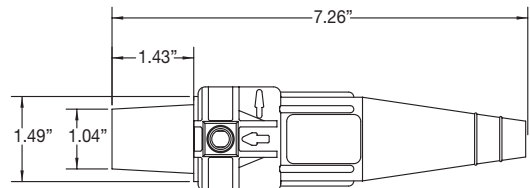
Female Connector
