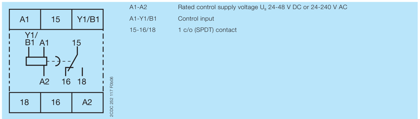
Connection diagram
