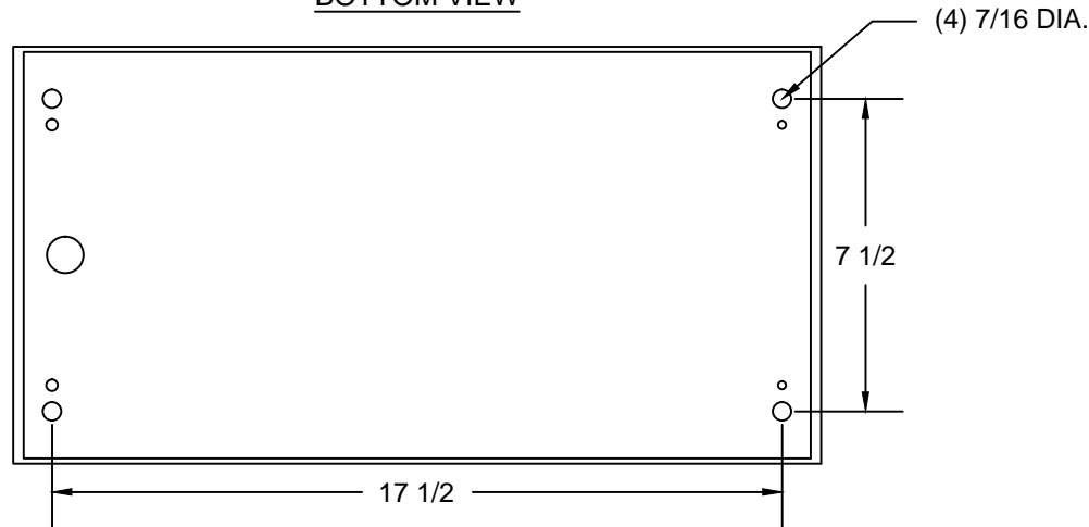
BOTTOM VIEW
