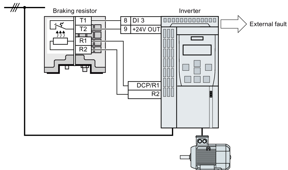
Figure 8-5 Connecting a braking resistor with temperature monitoring via digital input DI 3
