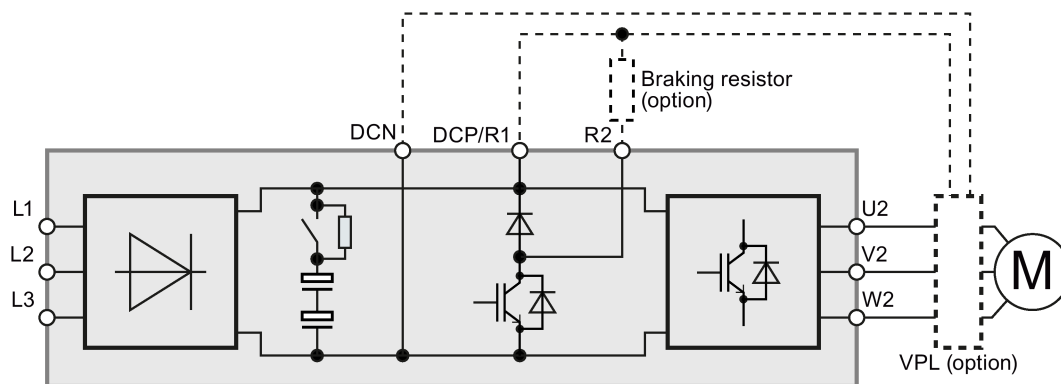
Figure 4-3 Block diagram of the inverter, FSA ... FSC
